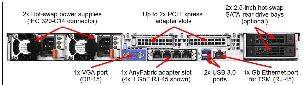
Figure 4. RD550 3.5-inch drive bay model rear view
