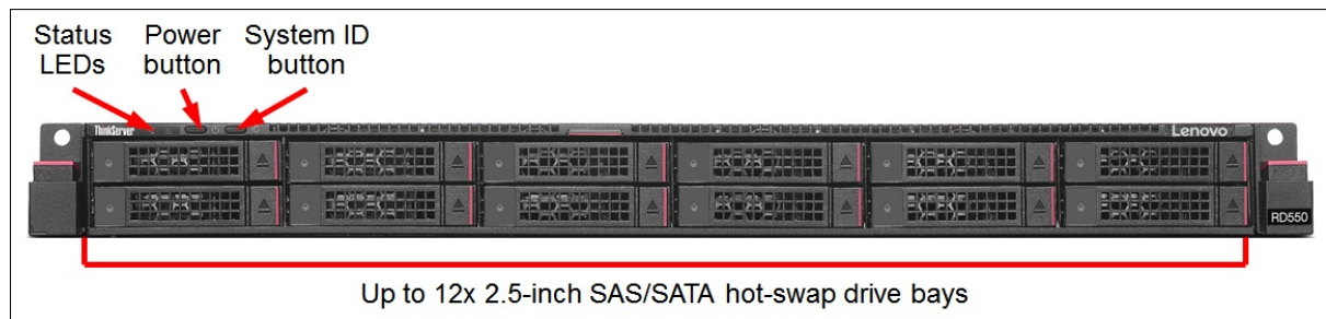
Figure 3. RD550 2.5-inch drive bay model front view
