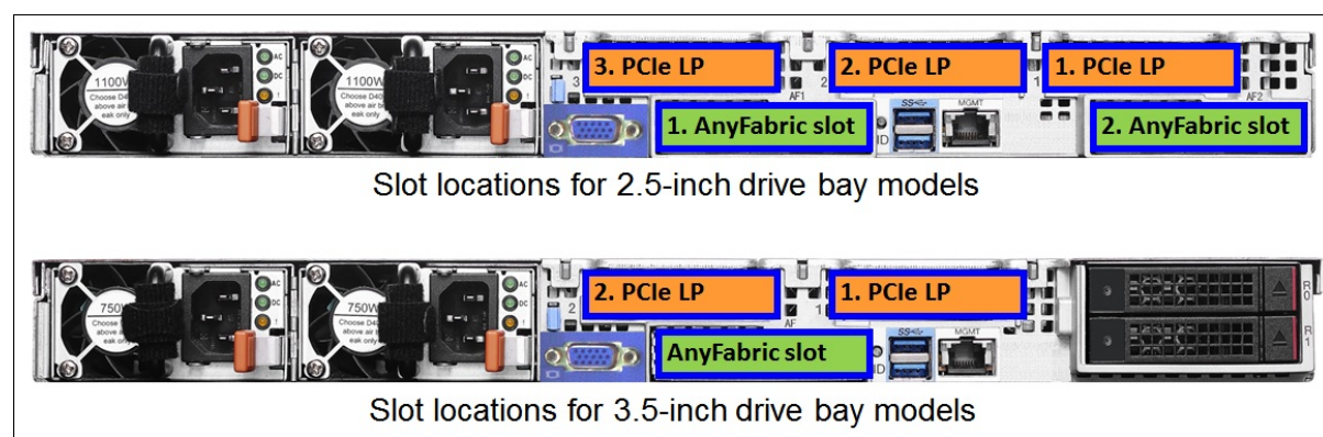
Figure 9. Slot locations
