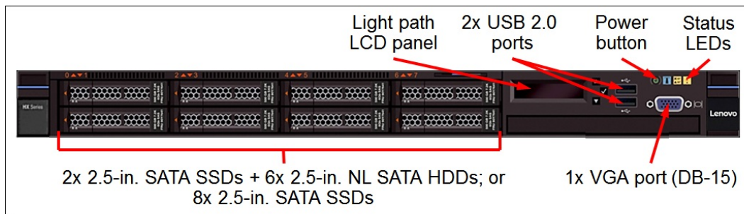
Figure 3. HX1310 front view
