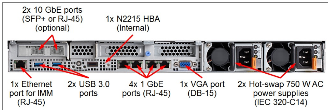
Figure 4. HX1310 rear view
