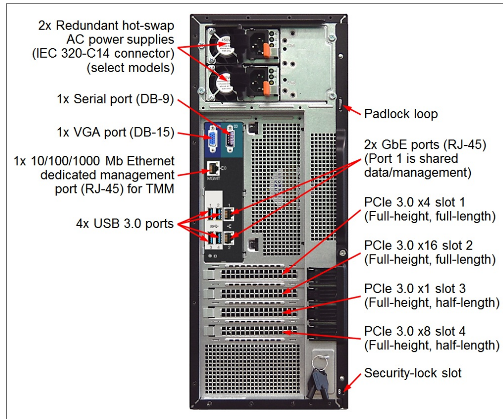
Figure 3. ThinkServer TS460 rear view
