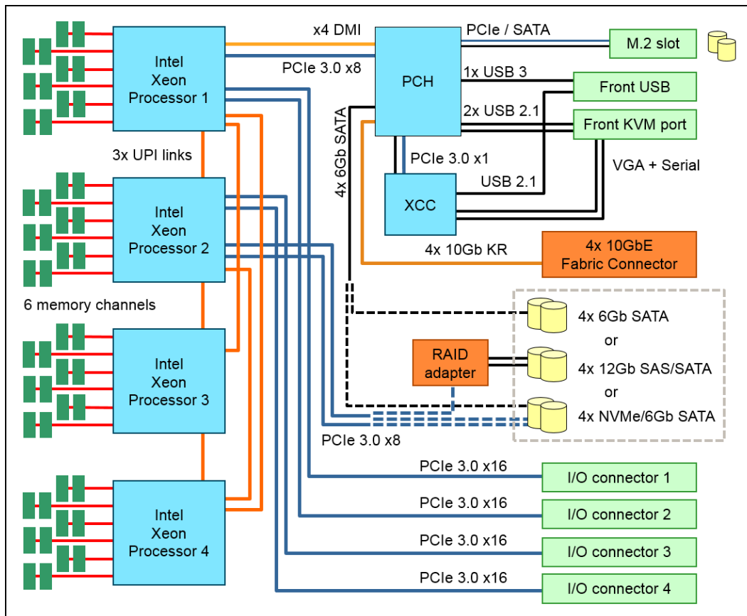
Figure 4. SN850 system architectural block diagram
