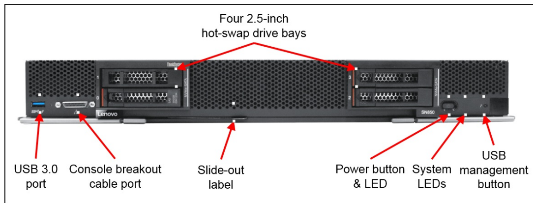
Figure 2. Front view of the SN850 server
