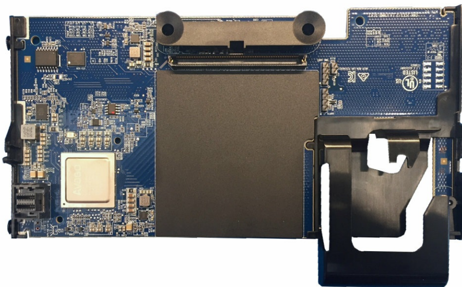
Figure 5. ThinkSystem RAID 530-4i
