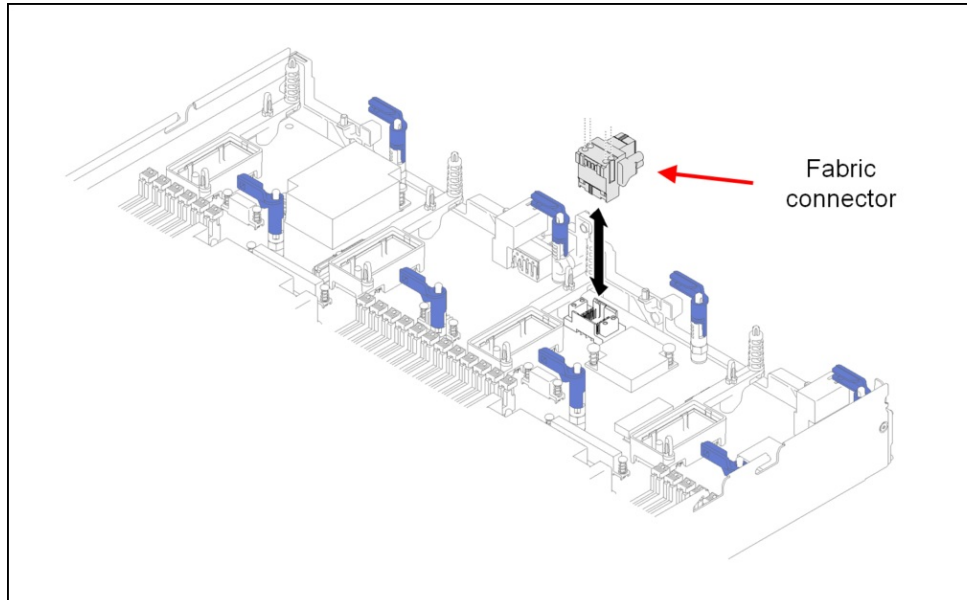
Figure 6. Location of fabric connector in SN850 server
