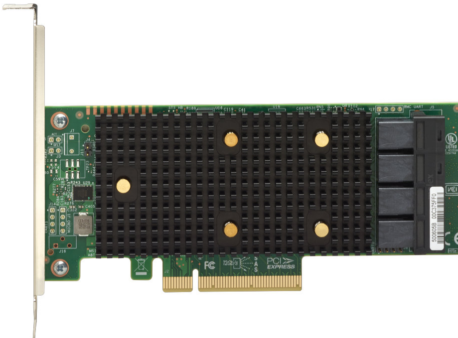
ThinkSystem 430-16i SAS/SATA 12Gb HBA
