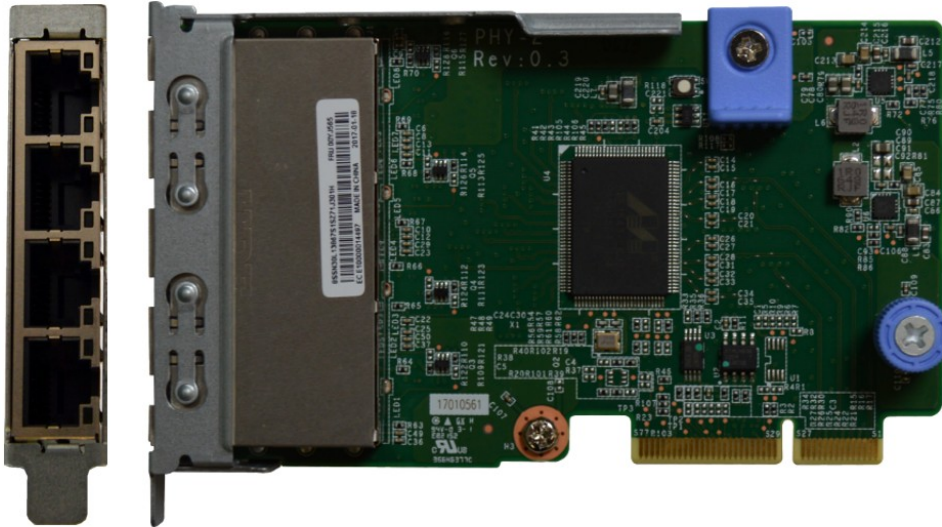
Figure 5. ThinkSystem 1Gb 4-port RJ45 LOM
