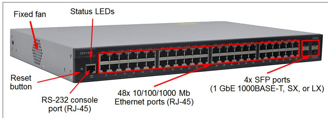
Figure 2. Front panel of the CE0152T Switch
