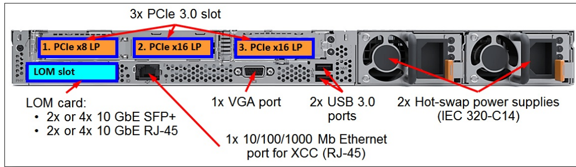
Figure 3. HX2320-E rear view
