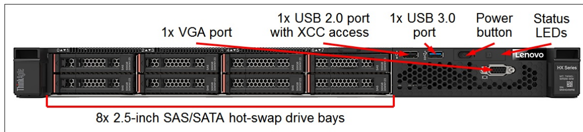
Figure 2. HX2320-E front view
