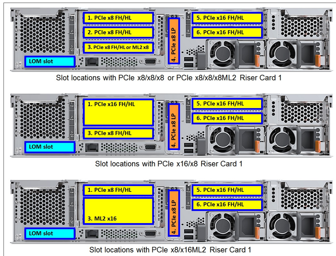
Figure 4. Slot locations
