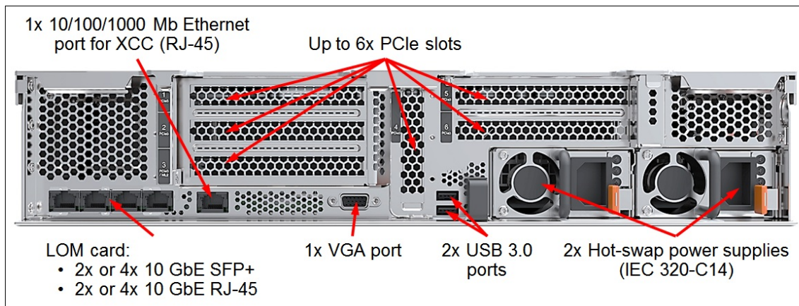
Figure 3. VX7520 rear view
