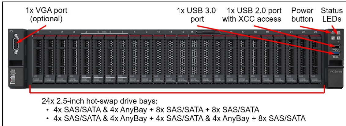
Figure 2. VX7520 front view
