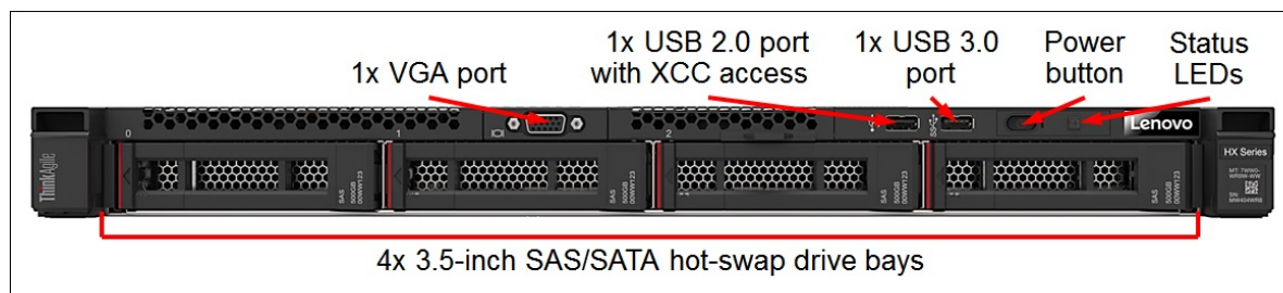
Figure 2. HX1321 front view
