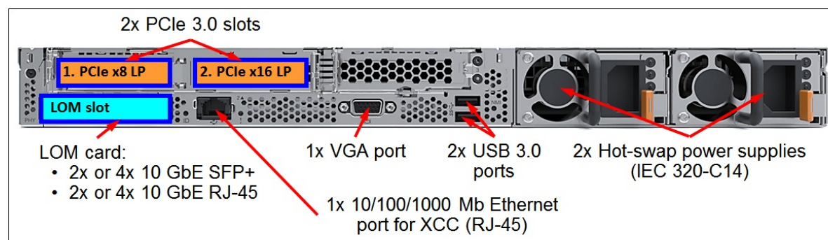
Figure 3. HX1321 rear view
