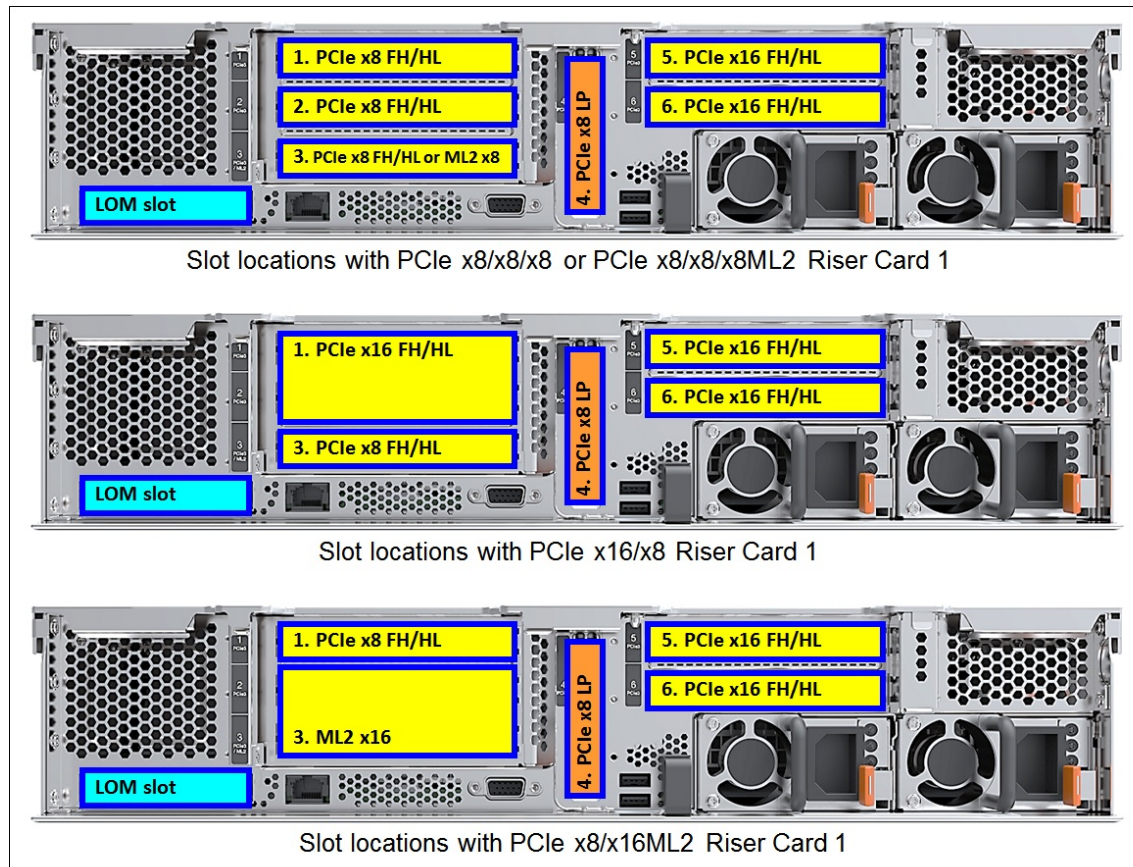
Figure 4. Slot locations
