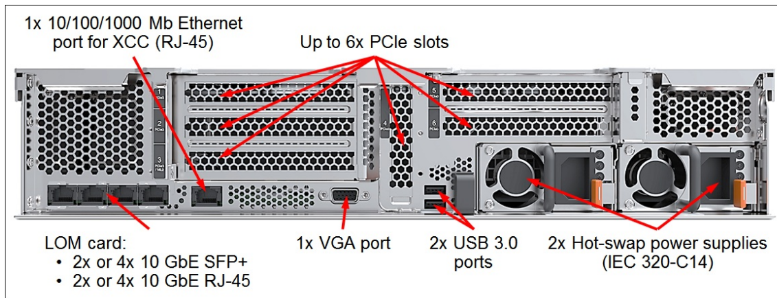
Figure 3. VX3520-G rear view
