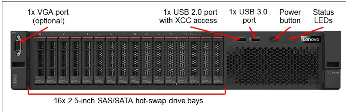
Figure 2. VX3520-G front view
