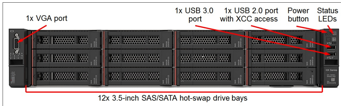
Figure 2. HX5520-C front view
