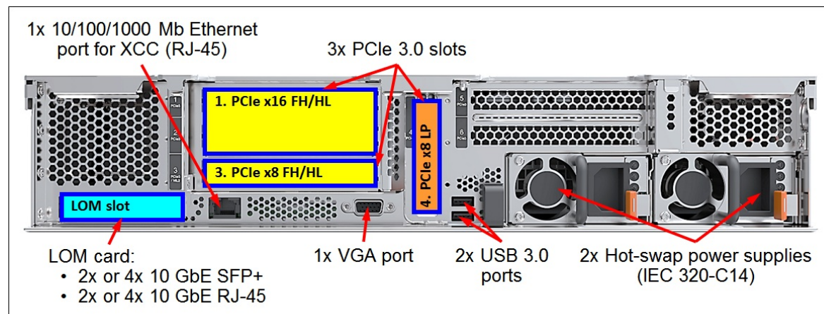
Figure 3. HX5520-C 12-drive bay appliance rear view
