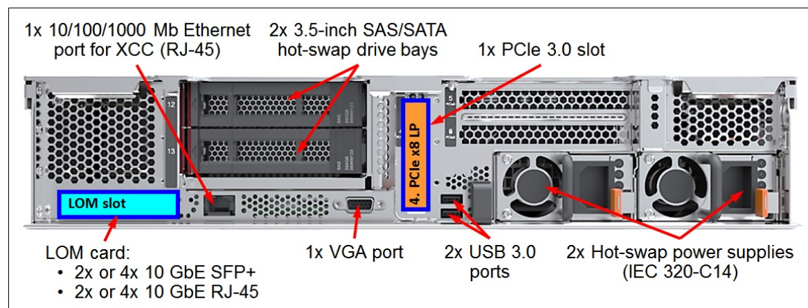
Figure 4. HX5520-C 14-drive bay appliance rear view
