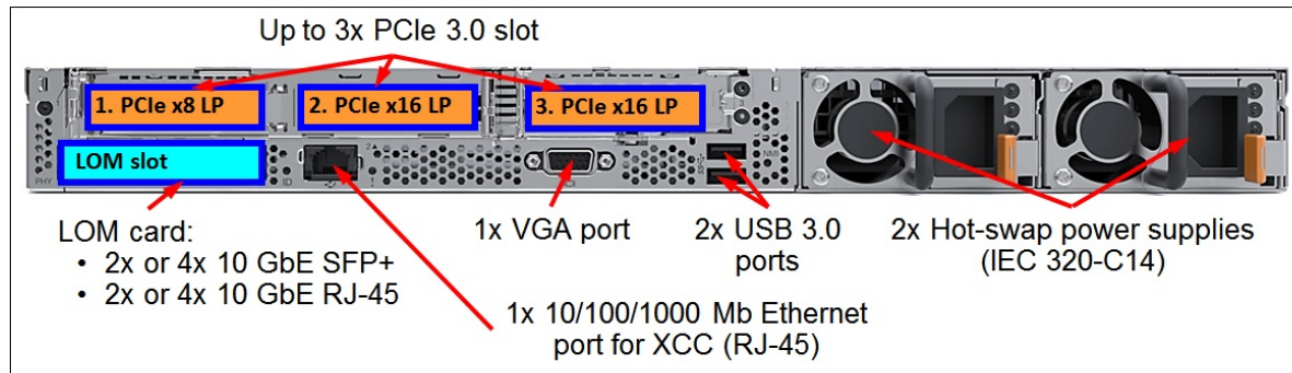
Figure 3. HX2321 rear view
