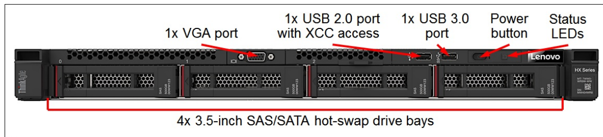
Figure 2. HX2321 front view
