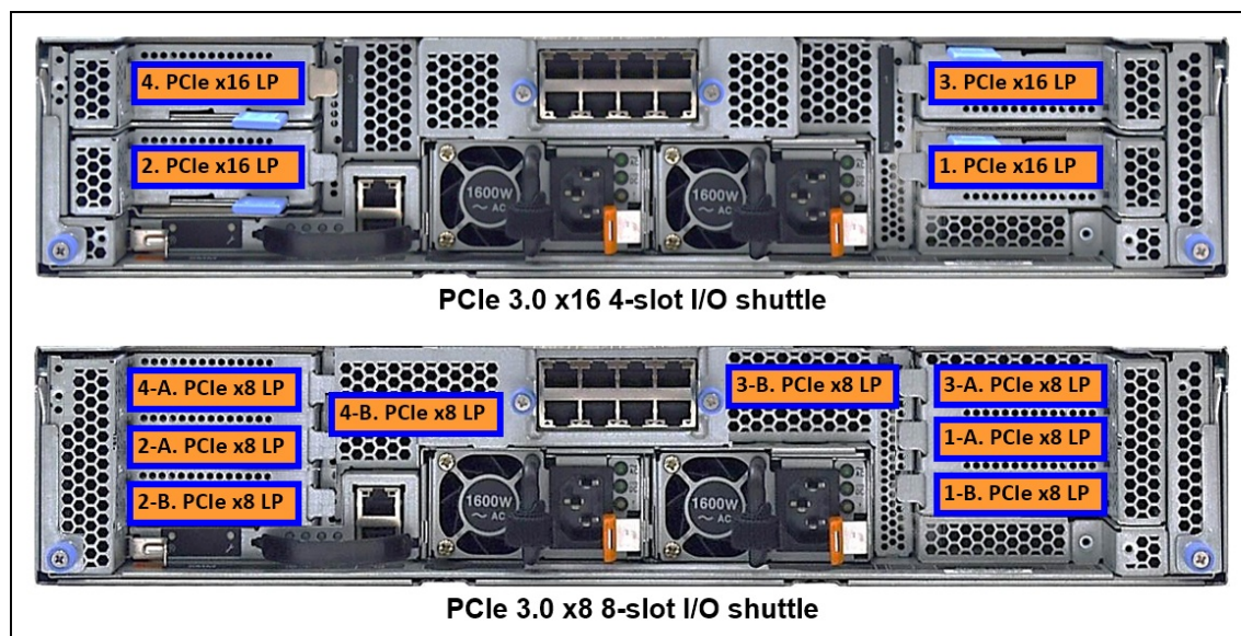
Figure 5. Slot locations
