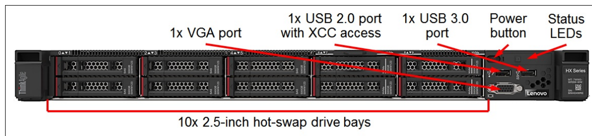
Figure 2. ThinkAgile HX3320 Appliance for SAP HANA front view
