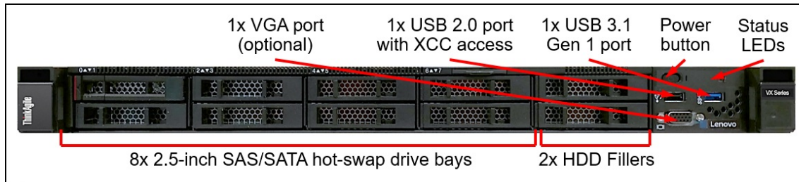
Figure 2. Front view of the ThinkAgile VX1320 appliance: 8x 2.5-inch drive bays
