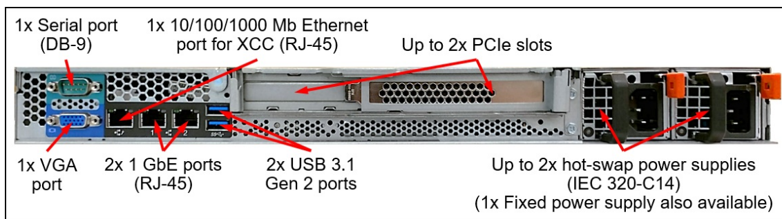
Figure 4. Rear view of the ThinkAgile VX1320 appliance
