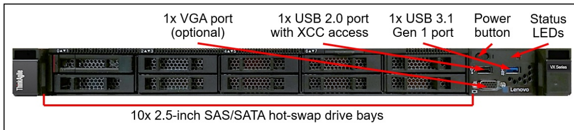
Figure 3. Front view of the ThinkAgile VX1320 appliance: 10x 2.5-inch drive bays
