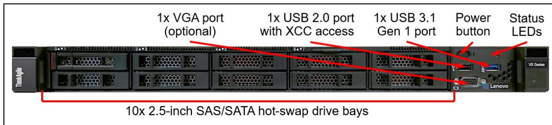
Figure 4. Front view of the VX 1SE Certified Node: 10x 2.5-inch drive bays
