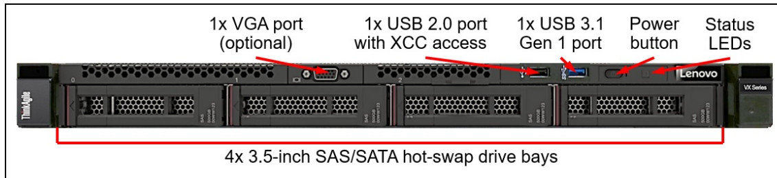
Figure 2. Front view of the ThinkAgile VX 1SE Certified Node: 4x 3.5-inch drive bays
