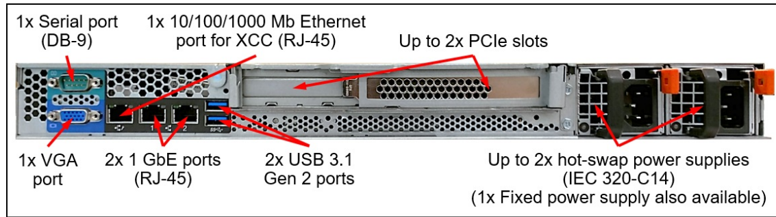
Figure 5. Rear view of the ThinkAgile VX 1SE Certified Node
