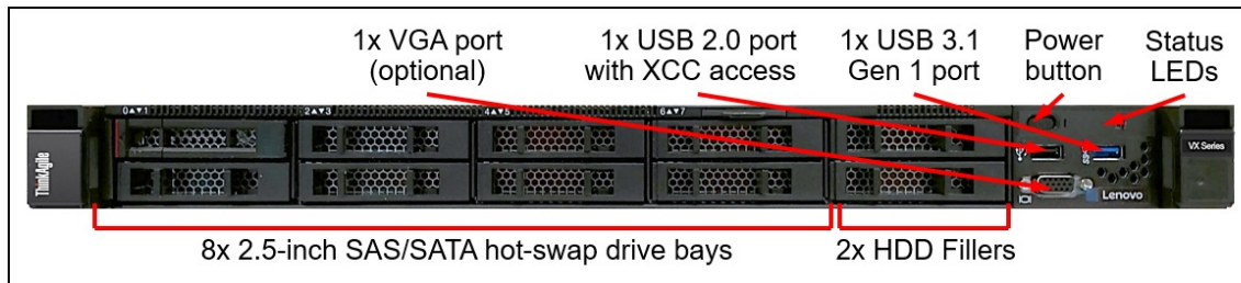
Figure 3. Front view of the ThinkAgile VX 1SE Certified Node: 8x 2.5-inch drive bays
