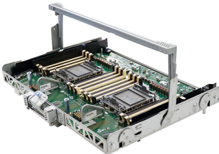
Figure 8. SR860 V2 Processor and Memory Expansion Tray
