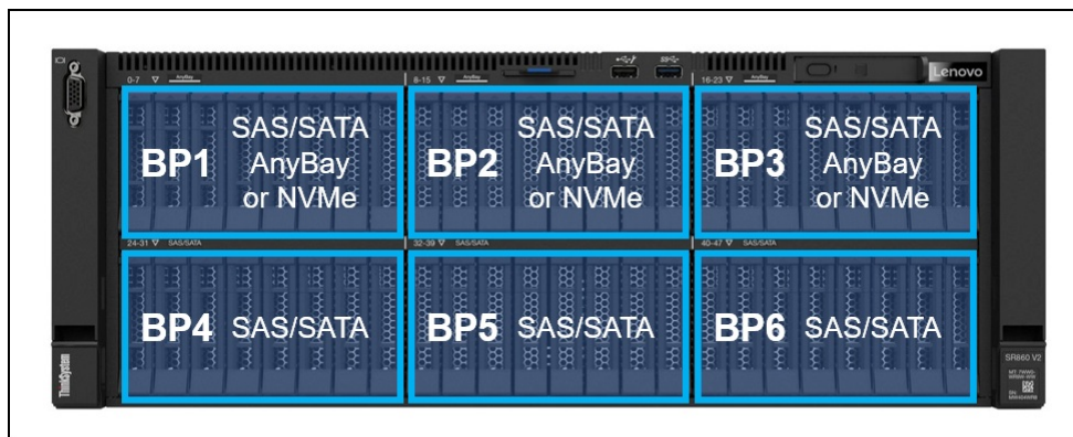
Figure 10. Backplanes
