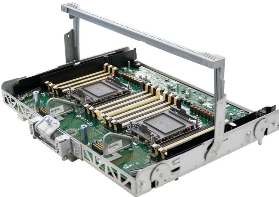
Figure 4. Processor and memory expansion tray
