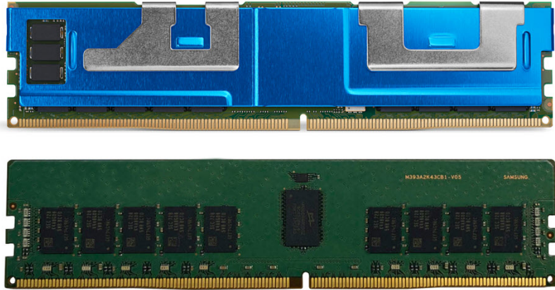
Figure 3. Intel Optane Persistent Memory 200 Series module (top) and standard memory DIMM (bottom)
