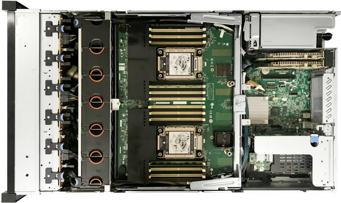
Figure 2. Internal view of the SR850 V2
