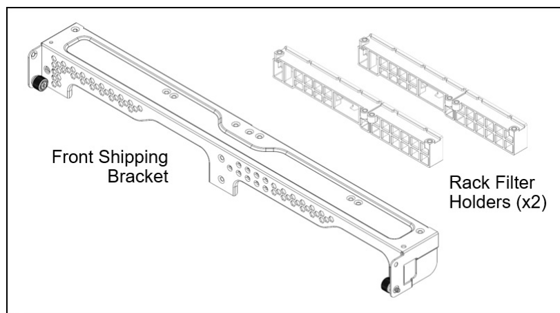
Figure 24. ThinkSystem Enclosure Front Shipping Bracket
