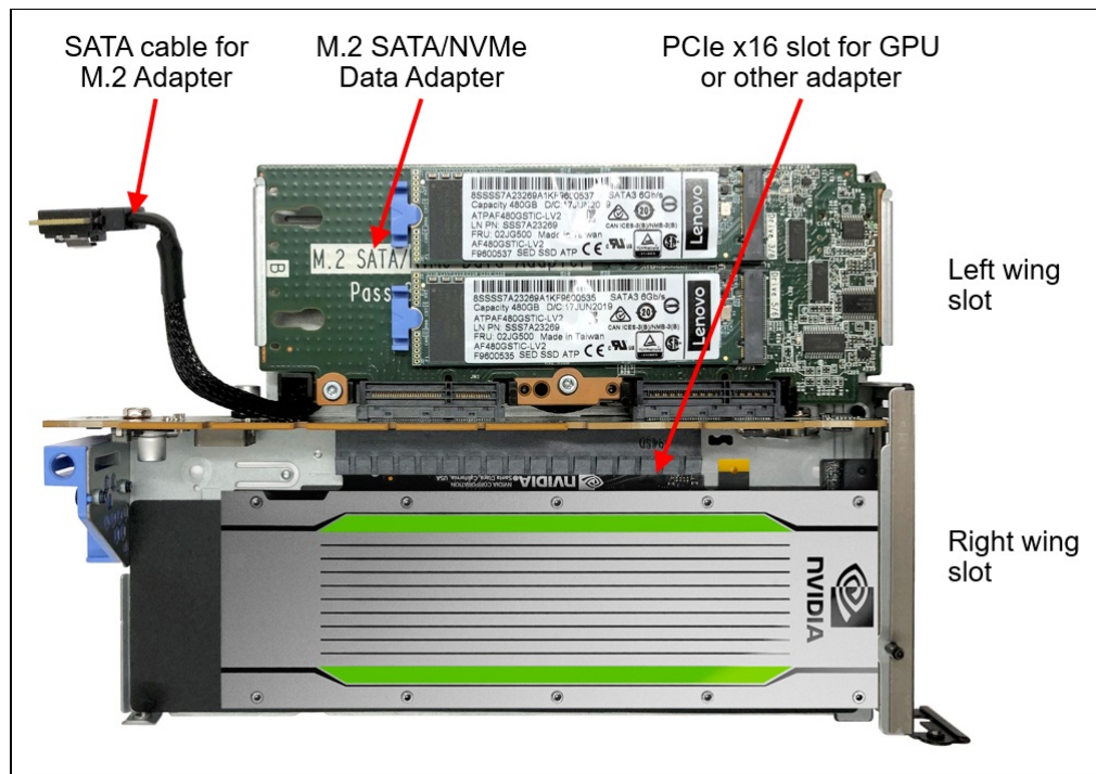
Figure 9. HX1021 PCIe Riser Cage (feature B6FD)
