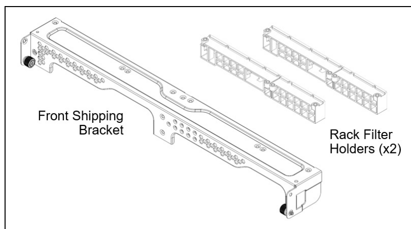
Figure 22. ThinkSystem Enclosure Front Shipping Bracket
