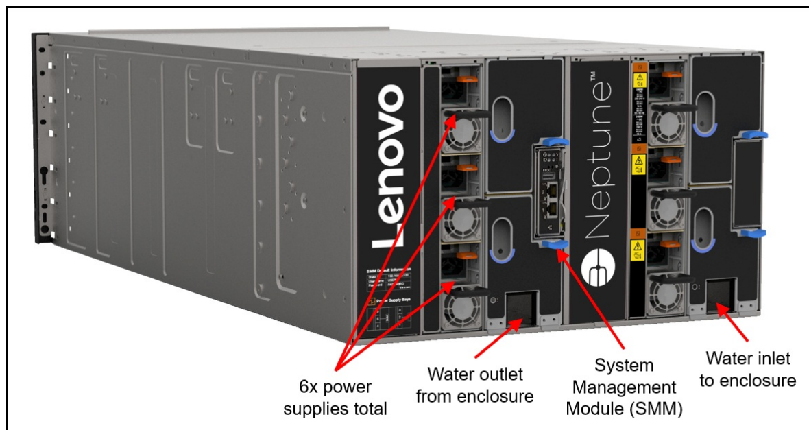
Figure 6. Rear view of the DW612 enclosure
