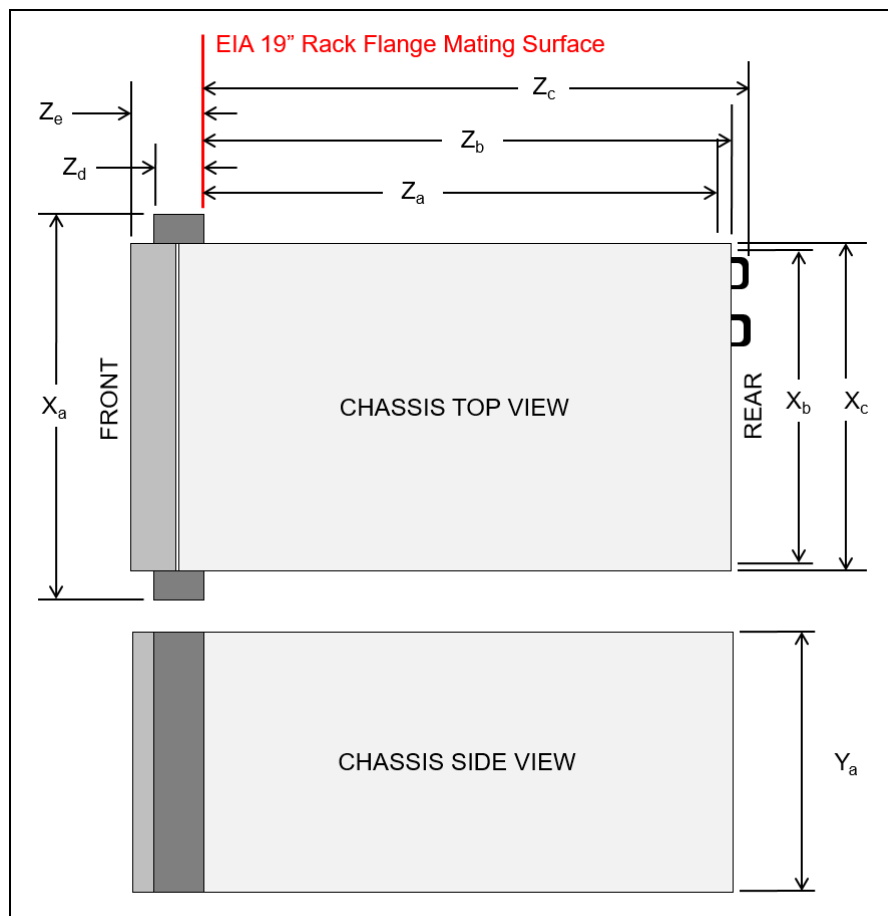
Figure 15. Enclosure dimensions
