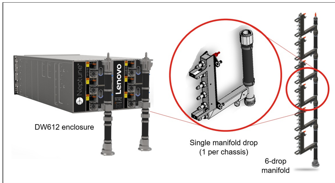
Figure 10. DW612 enclosure and manifold assembly
