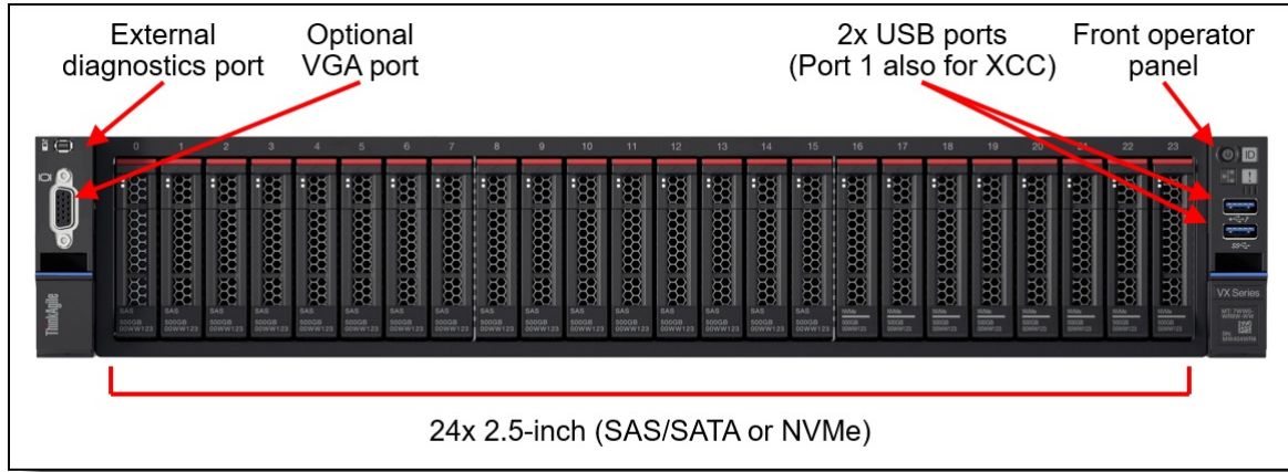
Figure 2. Front view of the ThinkAgile VX3575-G, VX7575 and VX7576 with 2.5-inch drives
