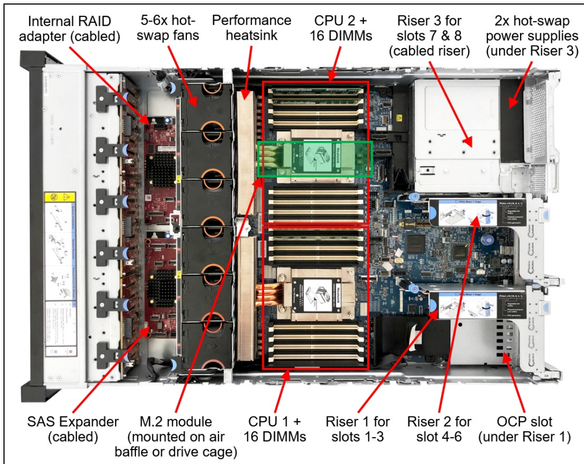
Figure 5. Internal view of the VX3575-G, VX5575, VX7575 and VX7576
