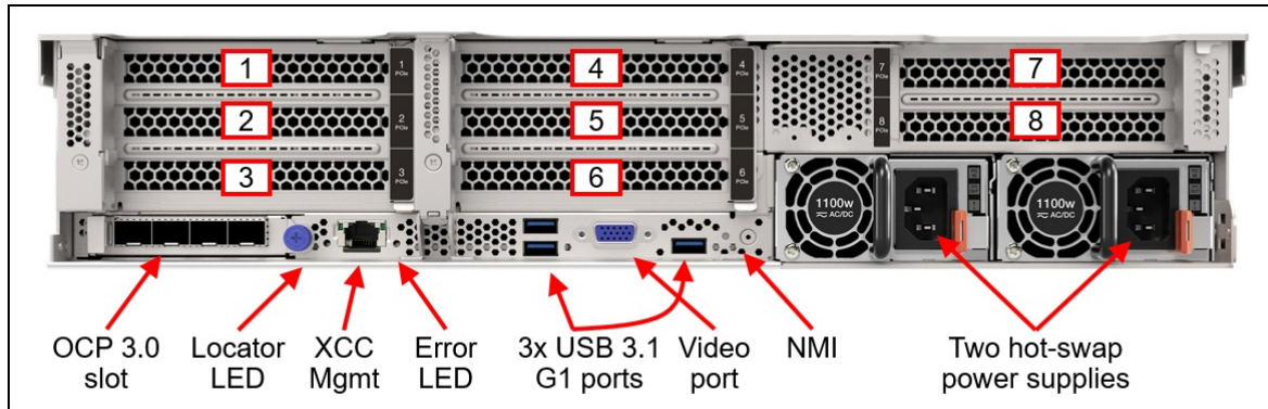
Figure 4. Rear view of the VX3575-G, VX5575, VX7575 and VX7576 (configuration with eight PCIe slots)
