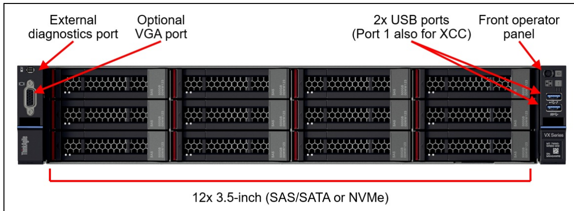
Figure 3. Front view of the ThinkAgile VX5575 and VX7576 with 3.5-inch drives
