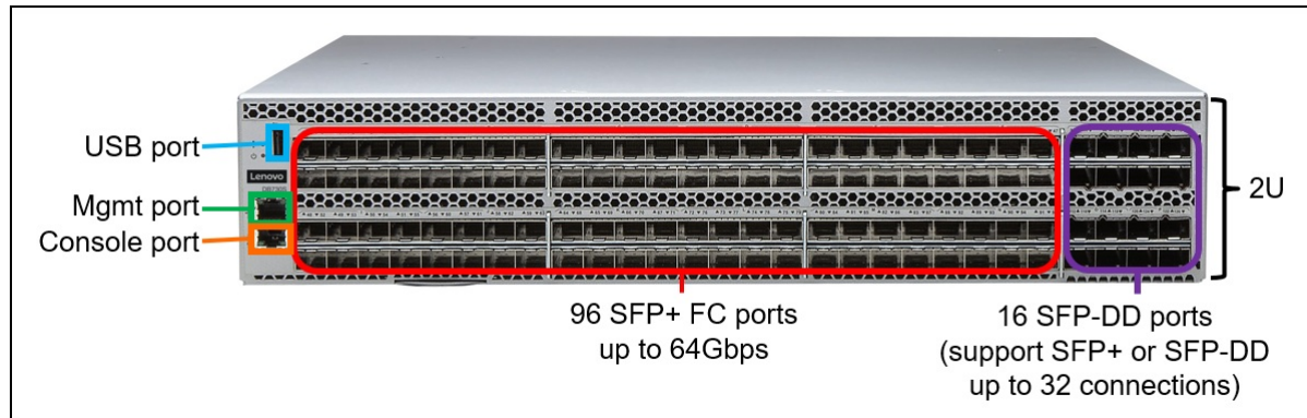
Figure 2. DB730S port-side view
