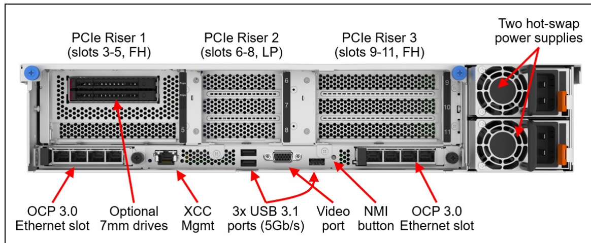
Figure 3. Rear view of the ThinkSystem SR850 V3
