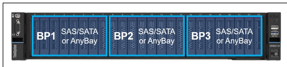
Figure 7. Backplanes
