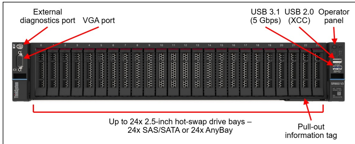
Figure 2. Front view of the ThinkSystem SR850 V3
