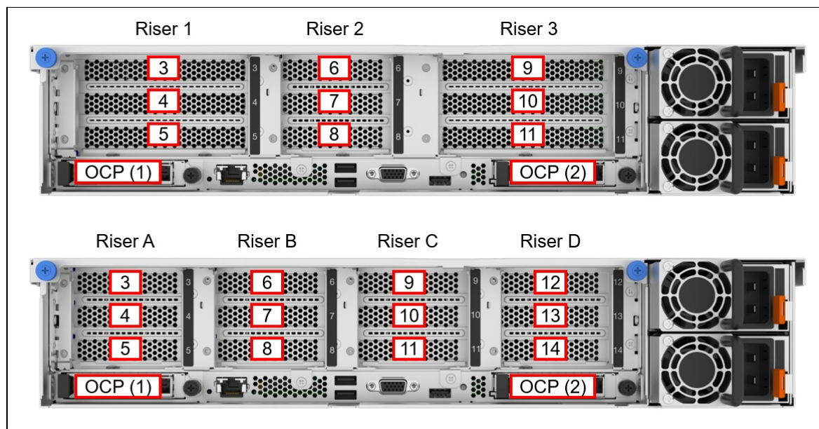
Figure 9. Slots in the SR850 V3
