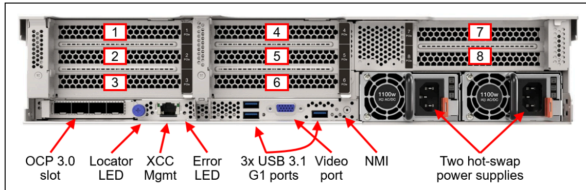
Figure 3. Rear view of the ThinkSystem SR665 V3 (configuration with eight full-height PCIe slots) The following figure shows the locations of key components inside the server.
