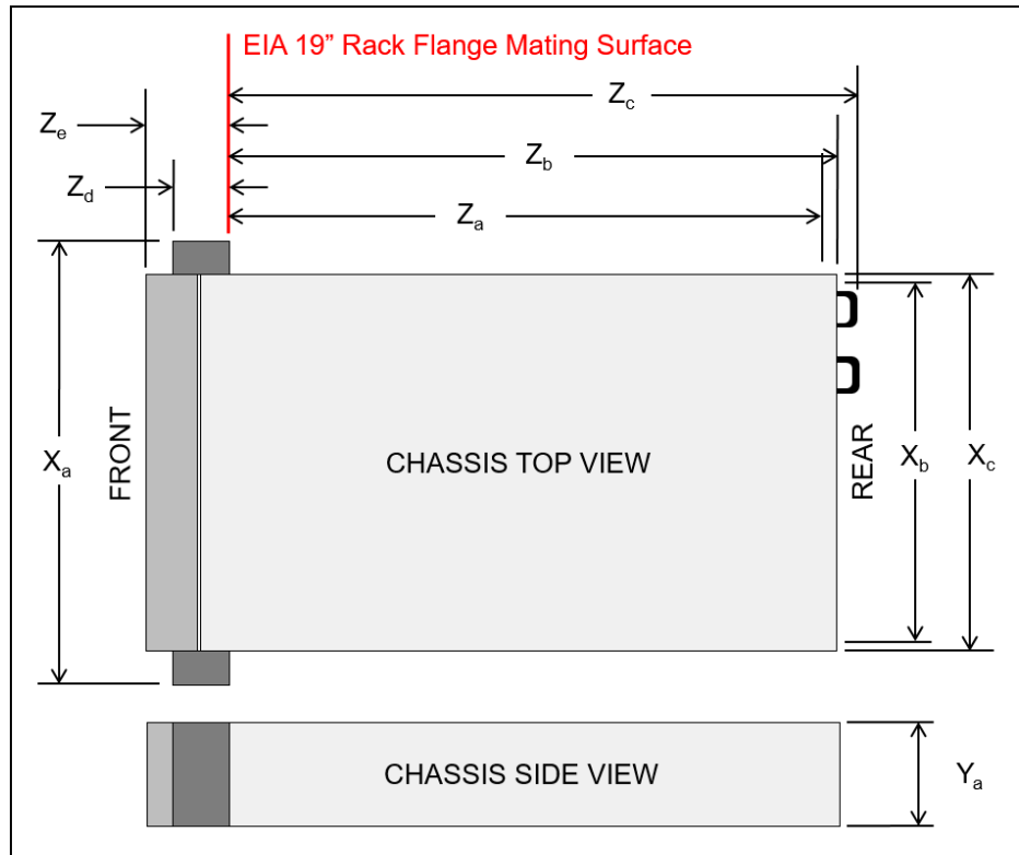
Figure 27. Server dimensions
