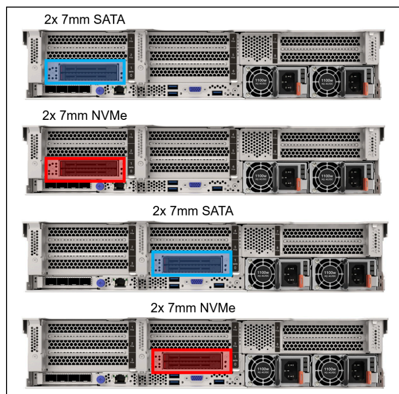
Figure 15. Rear 7mm drive bay configurations
