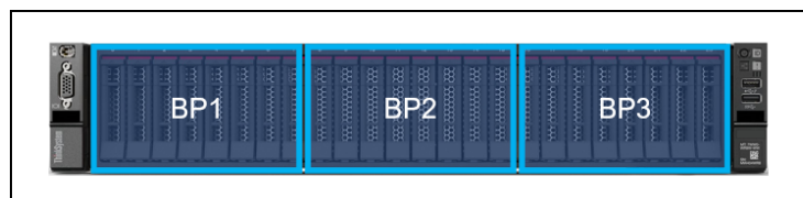
Figure 14. Backplane numbering
