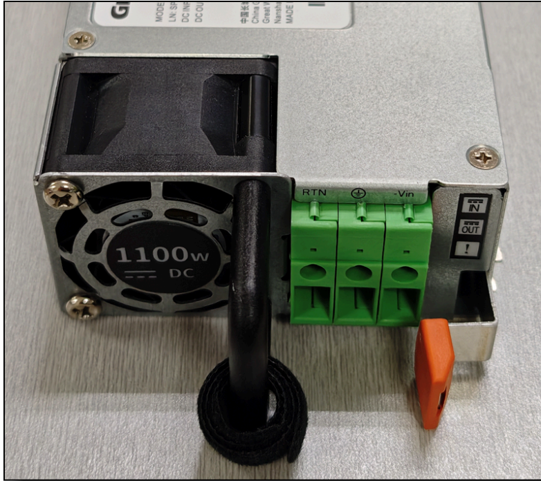
Figure 20. Connector on the ThinkSystem 1100W -48V DC Hot-Swap Gen2 Power Supply v2 (4P57A89415)
