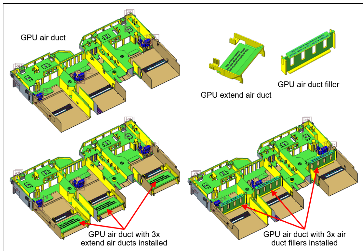
Figure 19. SR665 V3 GPU air duct
