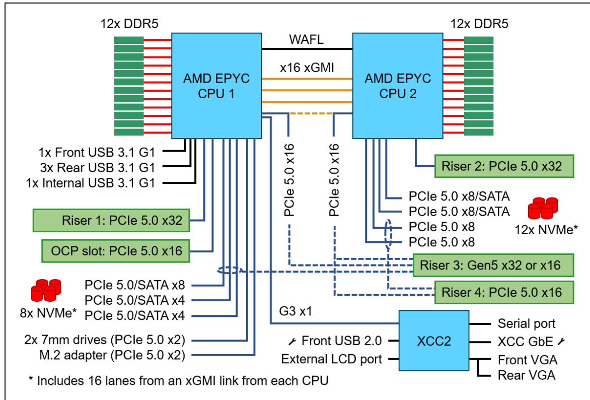
Figure 5. SR665 V3 system architectural block diagram
