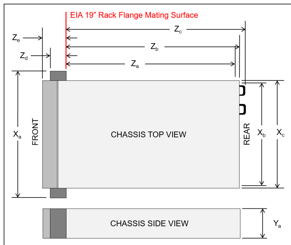
Figure 20. Server dimensions
