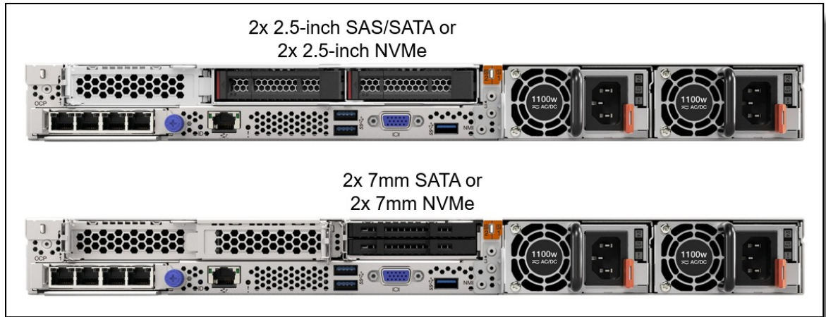
Figure 4.. Rear drive bay configurations of the SR630 V3
