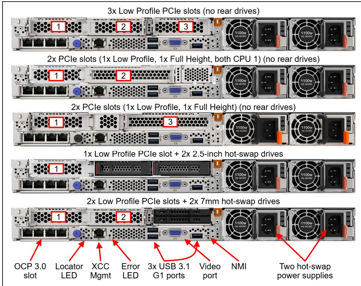
Figure 5. Rear view of the SR630 V3
