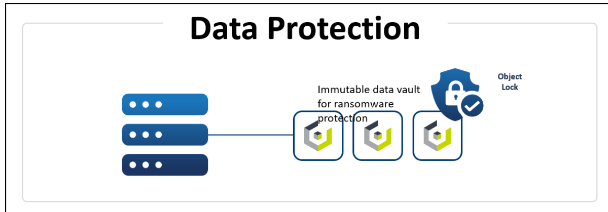
Figure 2. Data Protection
