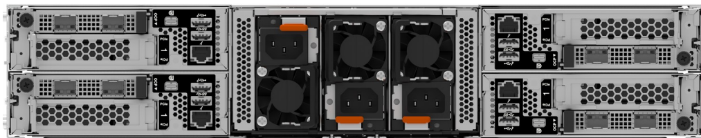
Figure 3. Rear View - SD530 V3 Nodes installed in D3 Chassis (with 2 PSUs)
