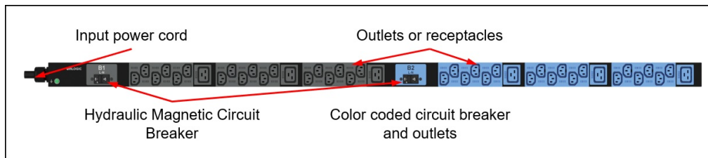
Figure 3. Connectors for Basic PDU (part number 4PU7A93169)
