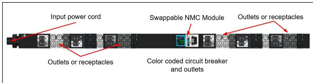
Figure 4. Connectors for Switched and Monitored PDU (part number 4PU7A93175)
