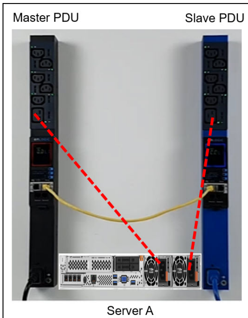
Figure 8. RNA setup with LAN
