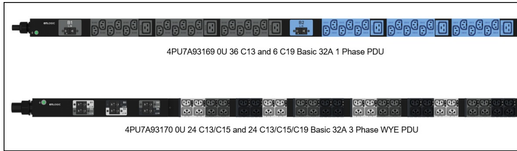
Figure 1. Lenovo 0U Basic PDUs
