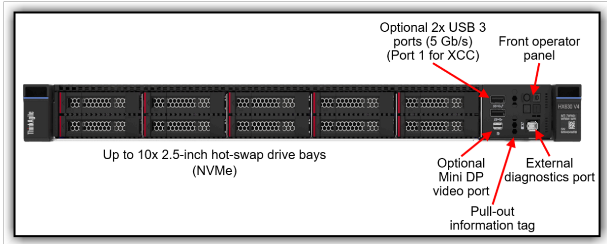
Figure 2. Front view of the HX630 V4 with 2.5-inch drives
