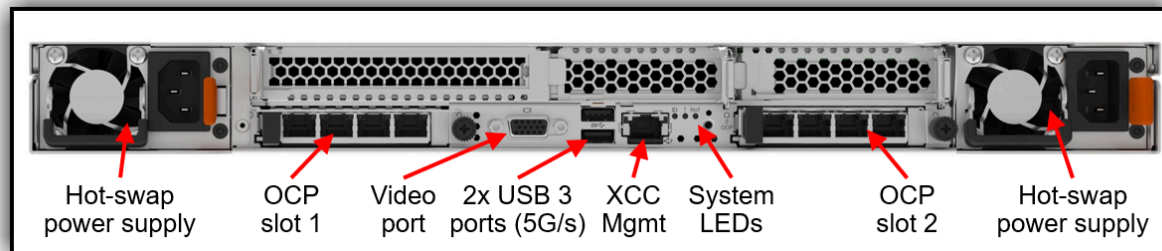
Figure 3. Rear views of the HX630 V4
