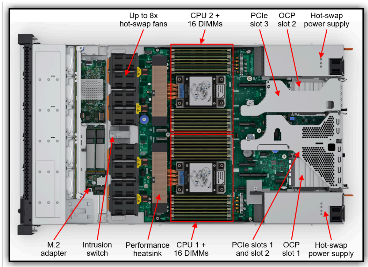
Figure 4. Internal view of the HX630 V4 systems
