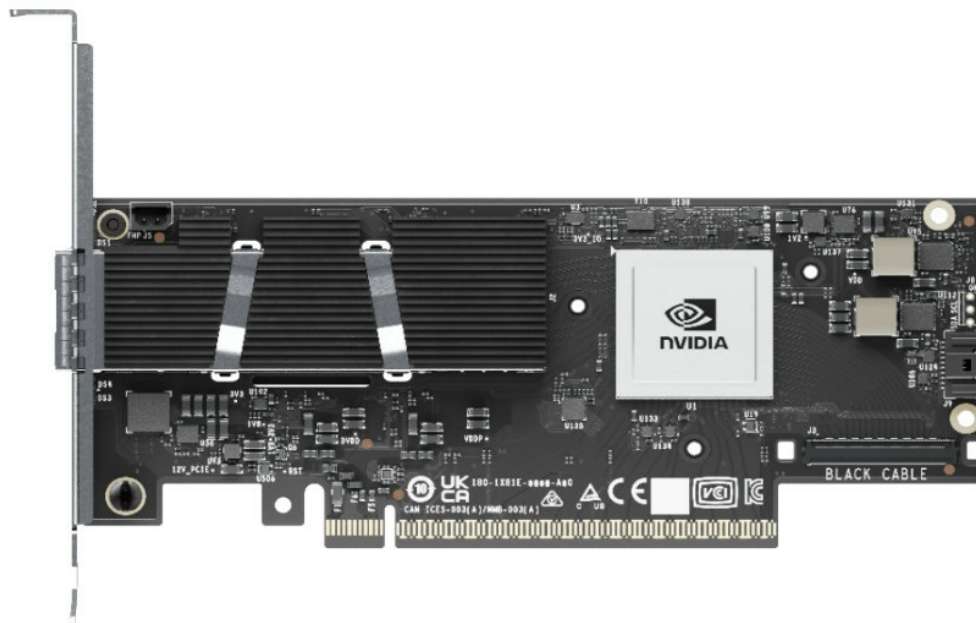
Figure 1. ThinkSystem NVIDIA ConnectX-8 8180 800Gbs OSFP PCIe Gen6 x16 Adapter (full-adapter gold case and heatsink removed)
