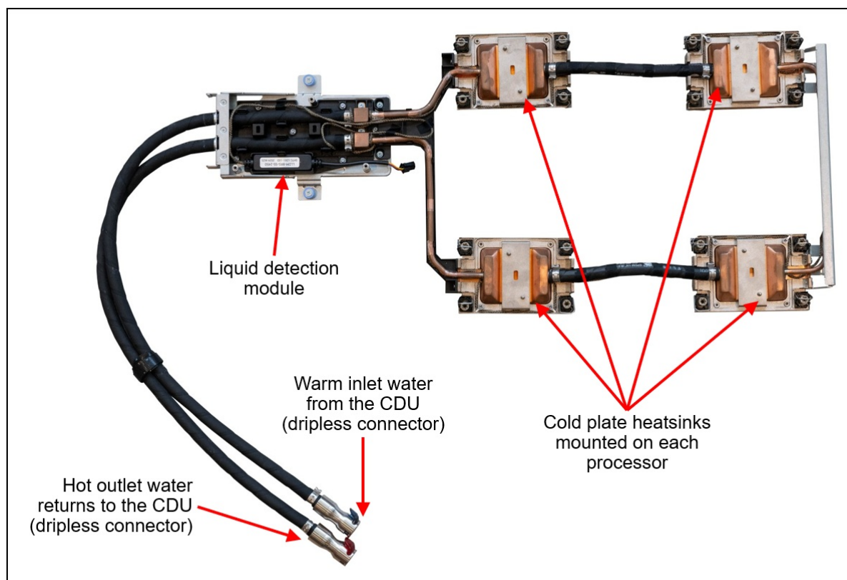
Figure 10. Lenovo Processor Neptune Core Module
