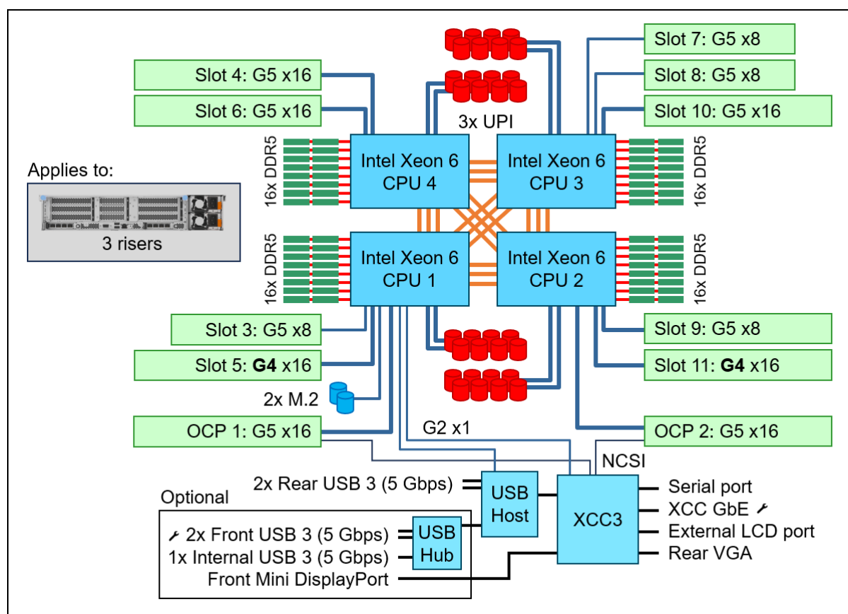
Figure 9. SR850 V4 system architectural block diagram - 3-riser configuration
