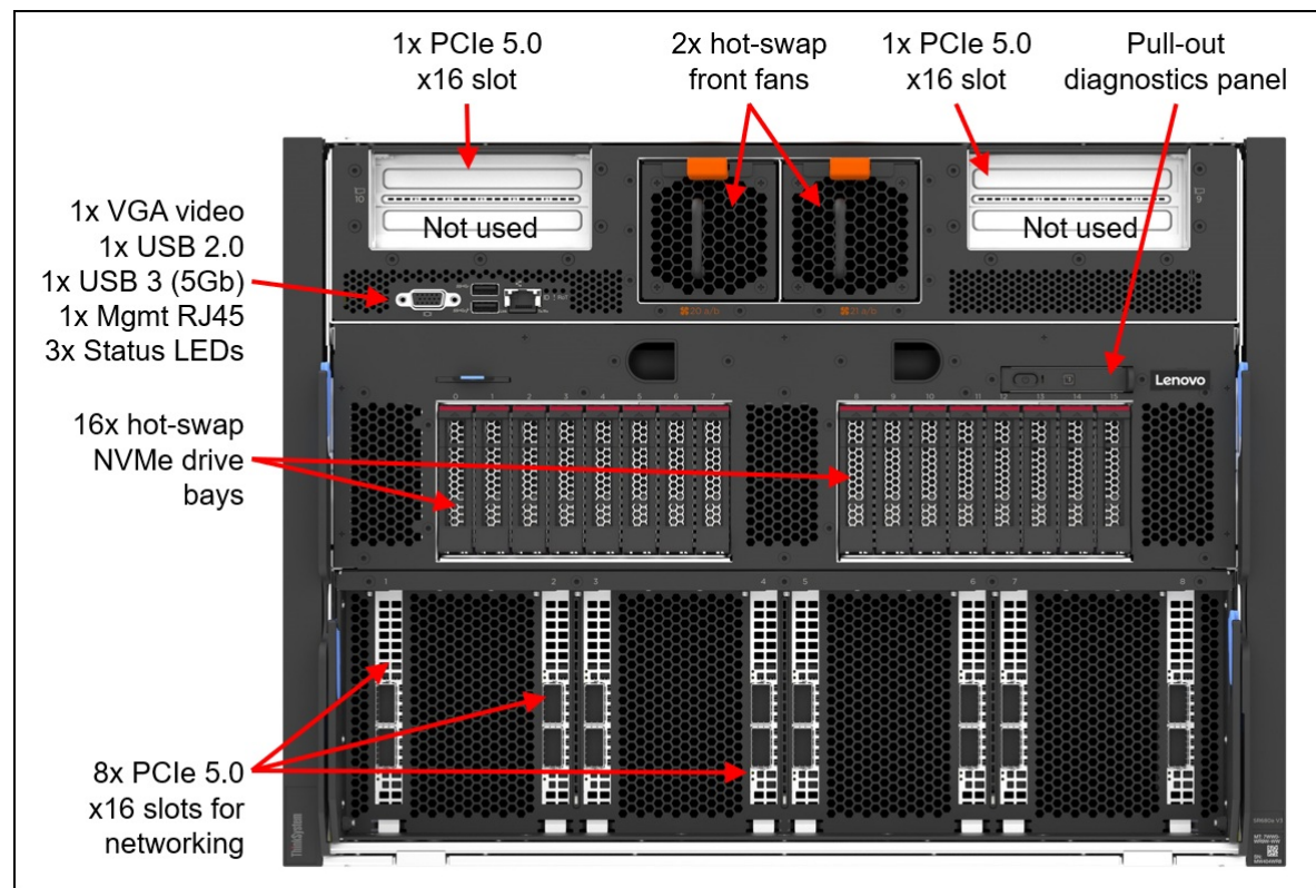
Figure 2. Front view of the ThinkSystem SR680a V3 with B200
