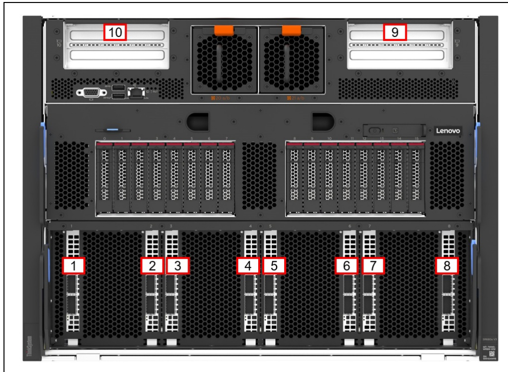
Figure 4. Slots of the SR680a V3 with B200
