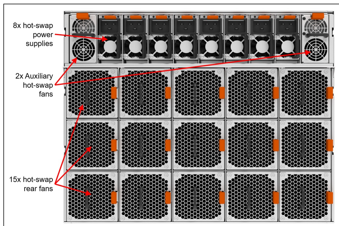
Figure 3. Rear view of the ThinkSystem SR680a V3 with B200
