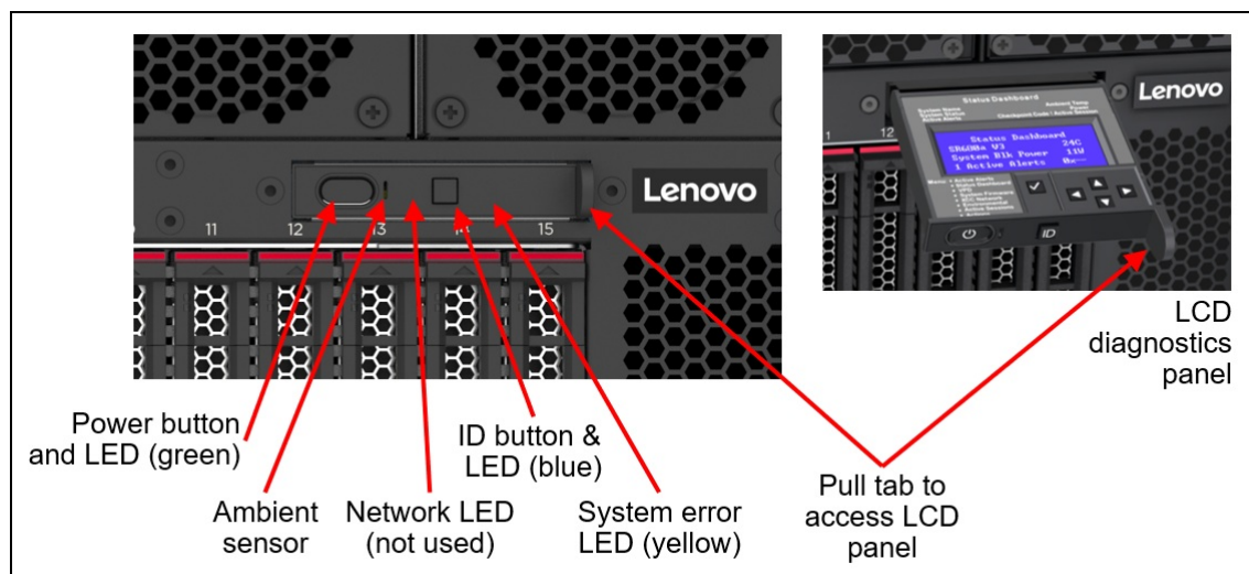
Figure 6. Front operator panel with pull-out diagnostics panel
