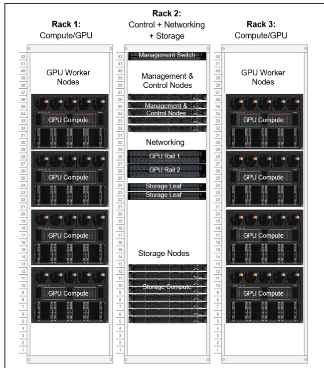
Figure 1. AI-DC Blueprint Solution Equipment Rack Layout example for 64 GPUs
