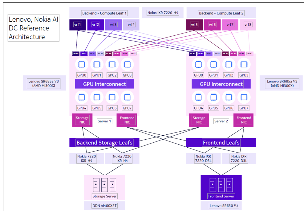
Figure 2. Lenovo, Nokia Sovereign AI Validated Design Architecture
