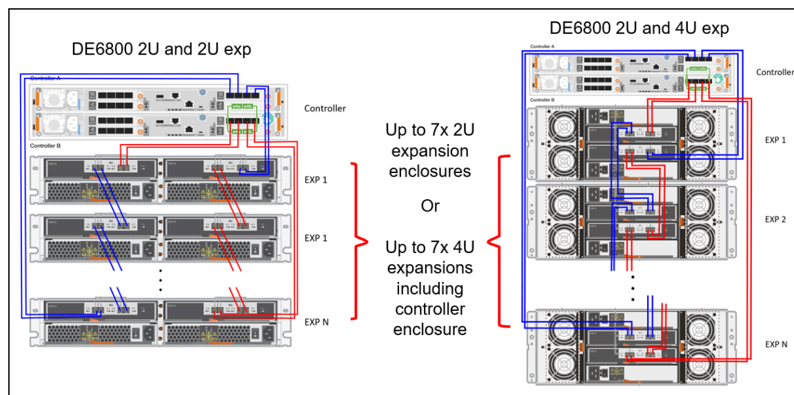
Figure 8. ThinkSystem DE6800 expansion enclosure connectivity topology
