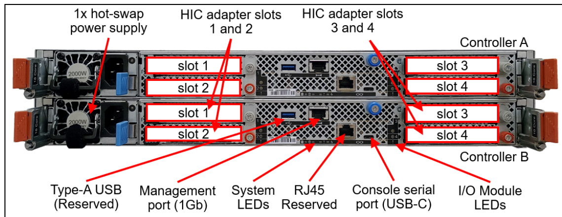
Figure 3. One controller of the ThinkSystem DE6800 2U SFF enclosure rear view
