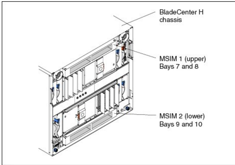
Figure 3. Two MSIMs installed in the BladeCenter H chassis
