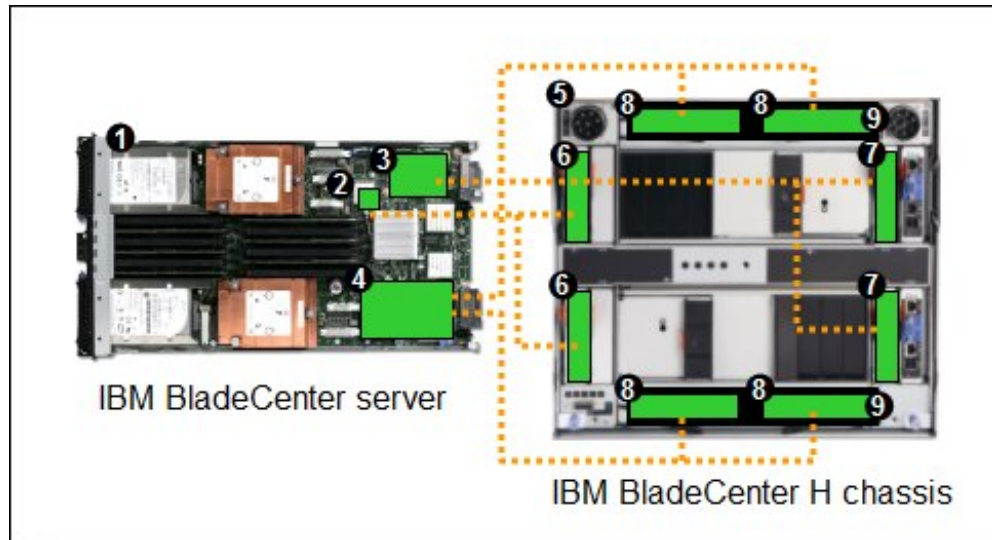
Figure 4. Using two MSIMs and eight Ethernet Switch Modules to route eight Ethernet ports per server
