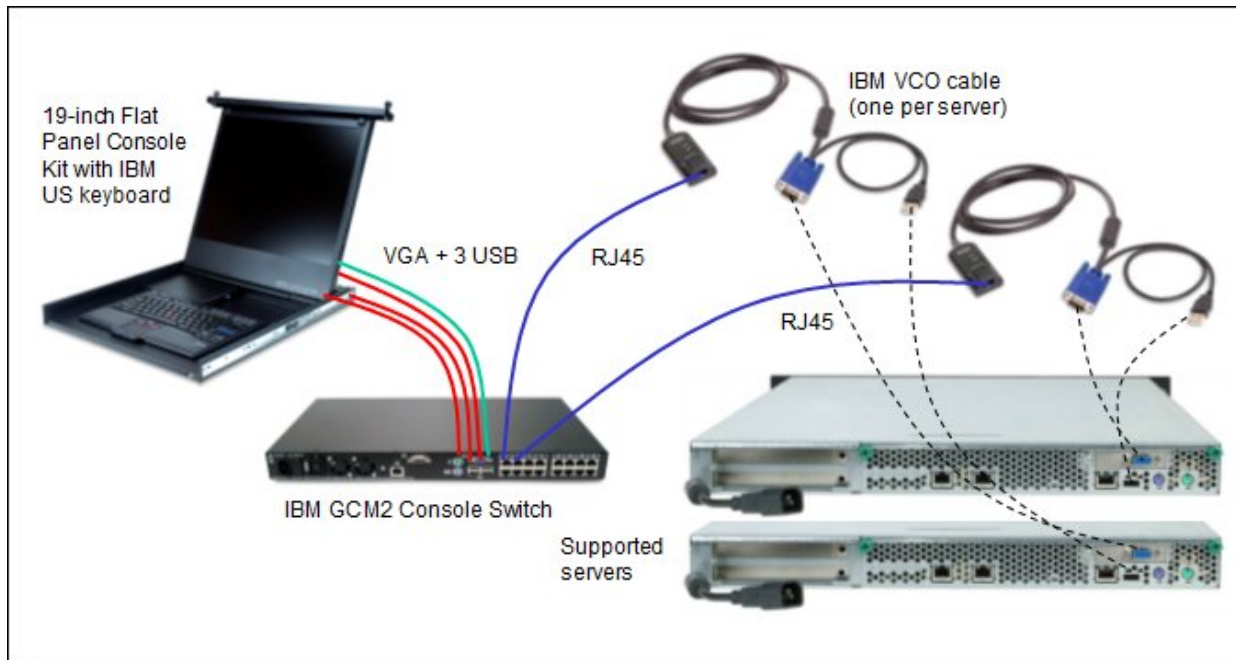
Figure 5. 19-inch Flat Panel Console Kit sample configuration
