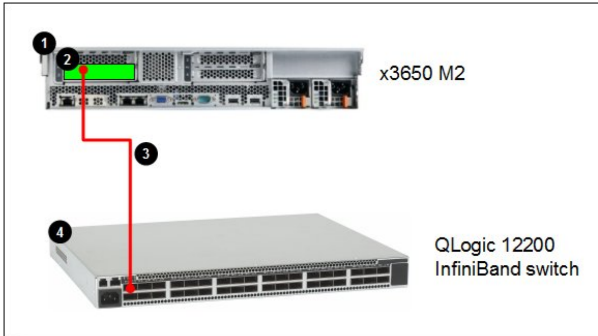
Figure 2. x3650 M2 server with the QLogic QLE7340 HCA connected to an InfiniBand network
