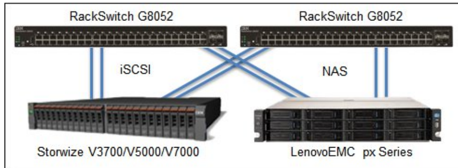
Figure 6. NAS and iSCSI
