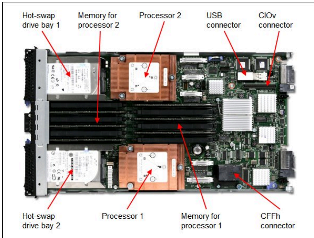
Figure 2. BladeCenter HS22
