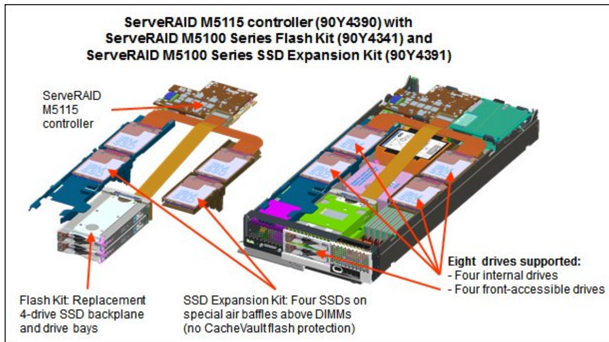
Figure 5. ServerRAID M5115 with Flash and SSD Expansion Kits installed
