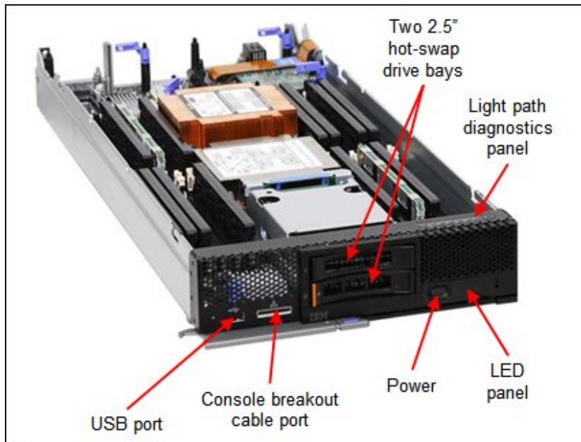
Figure 2. Front view of the Flex System x240 Compute Node
