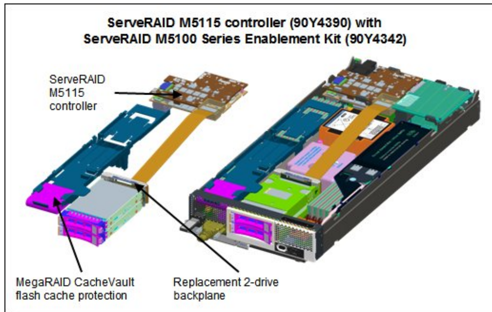
Figure 4. The ServerRAID M5115 and the Enablement Kit installed
