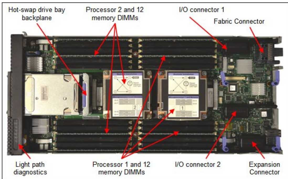
Figure 3. Inside view of the Flex System x240 Compute Node
