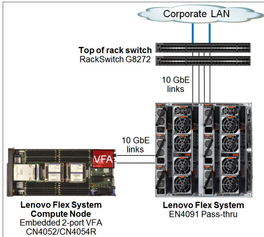
Figure 6. EN4091 in the 10 GbE network
