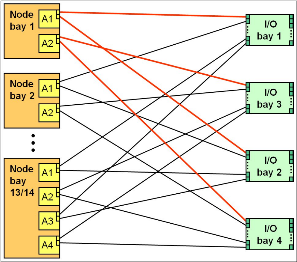
Figure 3. Logical layout of the interconnects between I/O adapters and EN4091 modules
