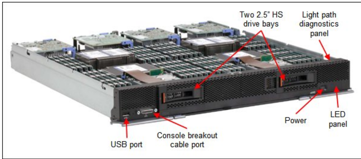
Figure 2. Front view of the Flex System x440 Compute Node
