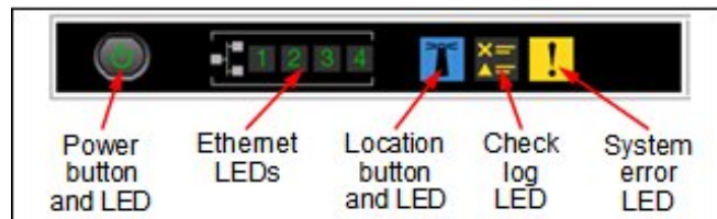
Figure 8. Basic (level 1) light path for models with eight drive bays
