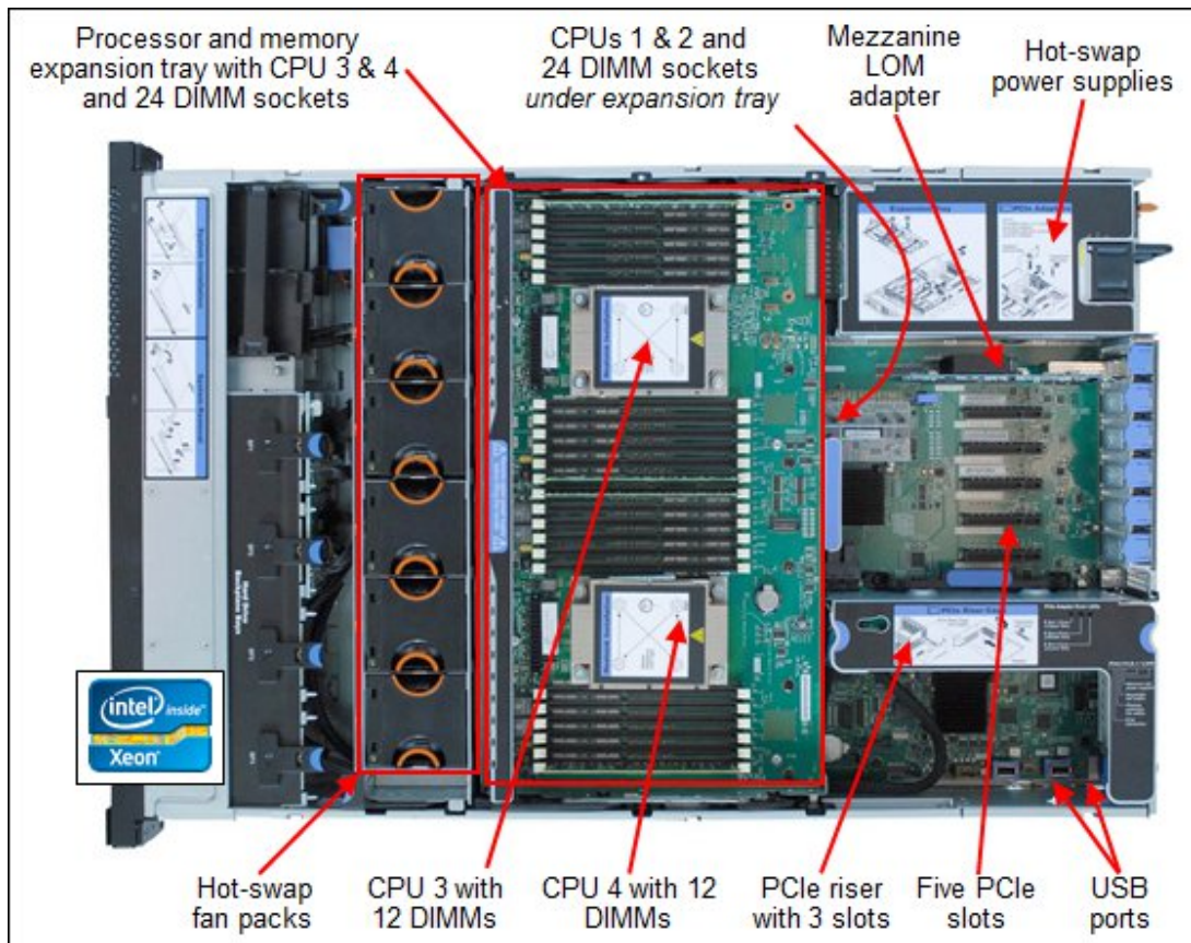
Figure 4. Inside view of the System x3750 M4 (machine type 8752)
