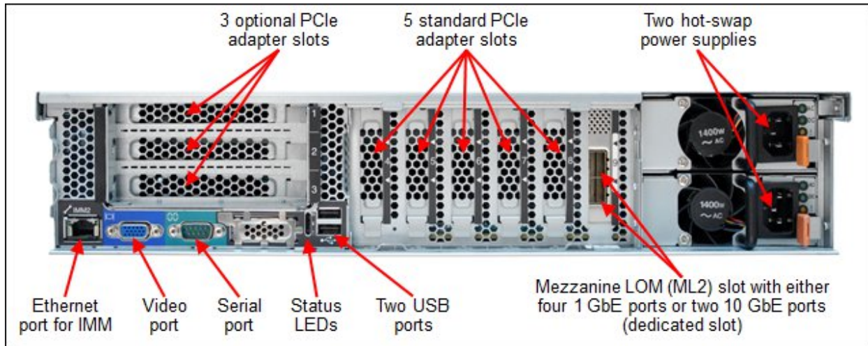
Figure 3. Rear view of the System x3750 M4 (machine type 8752)
