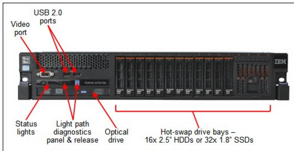
Figure 2. Front view of the System x3750 M4
