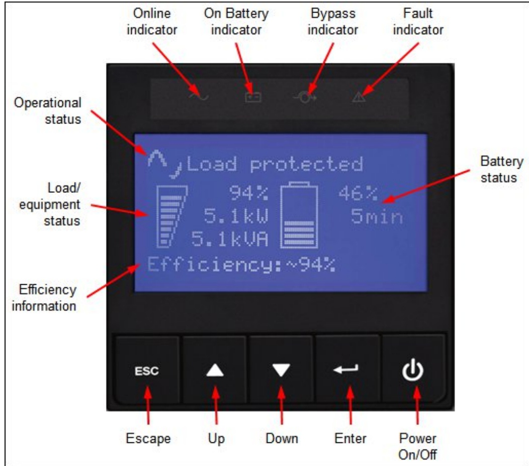
Figure 4. Control panel on the front of the RT5kVA or RT6kVA 3U Rack or Tower UPS
