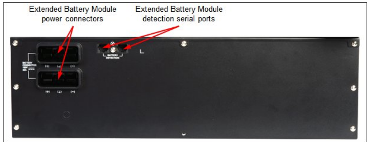
Figure 7. Rear view of the 5kVA/6kVA 3U Rack or Tower Extended Battery Module (55946BX)
