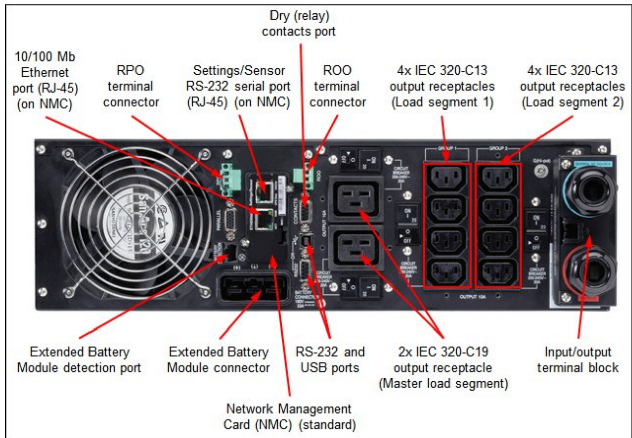
Figure 6. Rear view of the RT6kVA 3U Rack or Tower UPS (200-240VAC) (55946KX)
