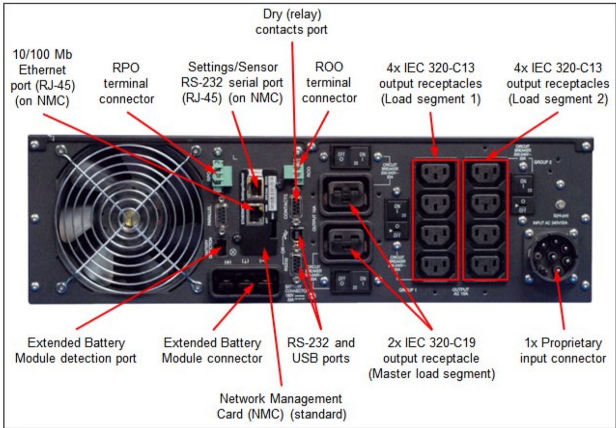
Figure 5. Rear view of the RT5kVA 3U Rack or Tower UPS (200-240VAC) (55945KX)
